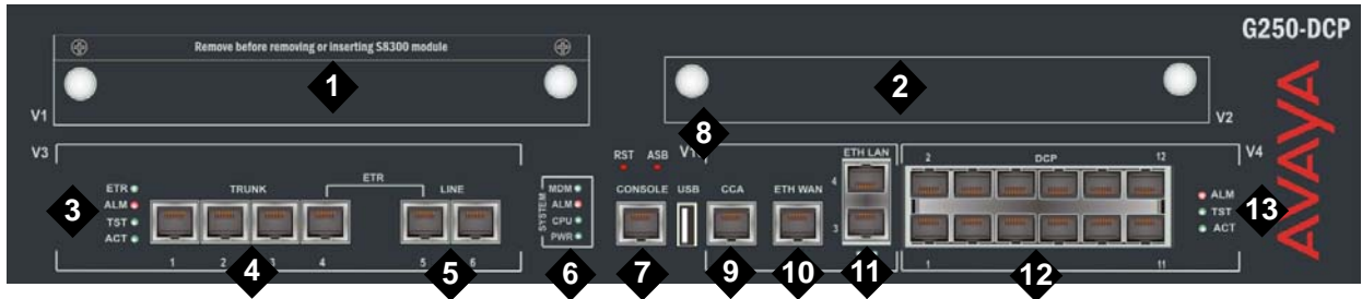
Figure 3: The Avaya G250-DCP Media Gateway Chassis
